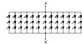
BACKLIGHT CIRCUIT DIAGRAM
